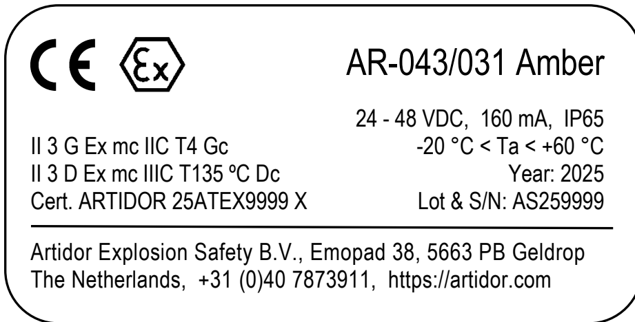
Example of an AR-043 signal light label
